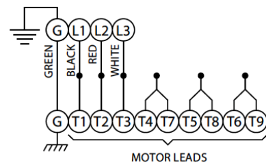
THREE-PHASE 460V AC POWER CORD 4x12
