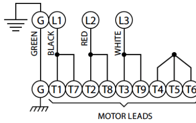
THREE-PHASE 208/230V AC POWER CORD 4x12
